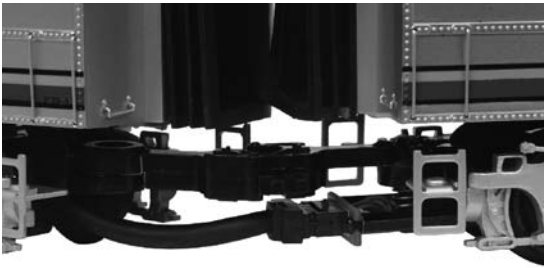
Figure 5: Correct way to Connect wire harness plug into the receptacle [The top of the plug will have the word 'TOP' imprinted on it]
