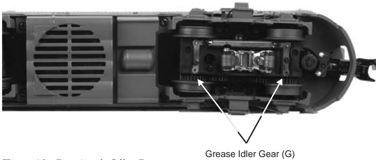
Figure 12: Greasing the Idler Gears
