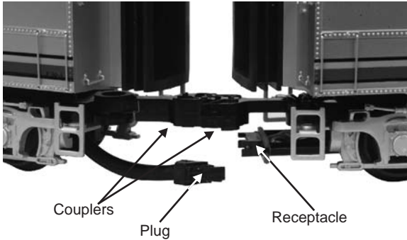
Figure 4: Connecting ABA Units
