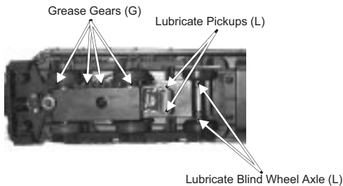
Figure 6: Lubricating The Locomotive Chassis
