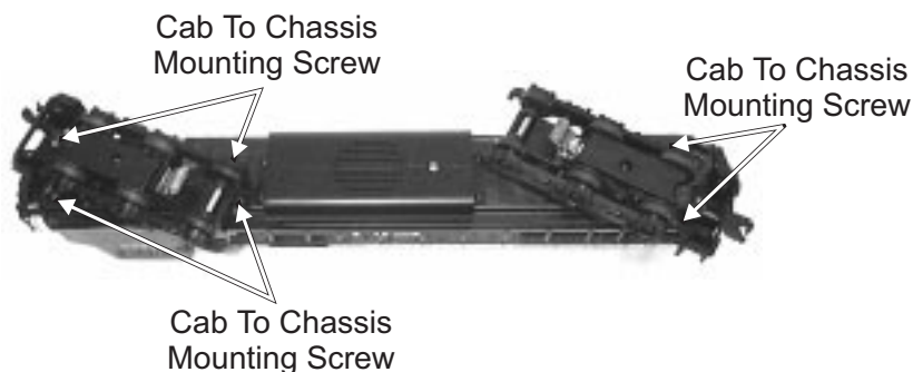
Figure 8: Removing The Body From The Chassis
