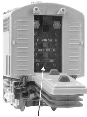
DCS/DCC Switch
