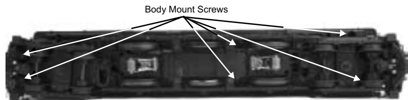
Figure 6. Body Removal Screw Locations
