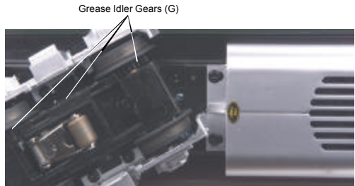
Figure 6: Greasing The Idler Gears
