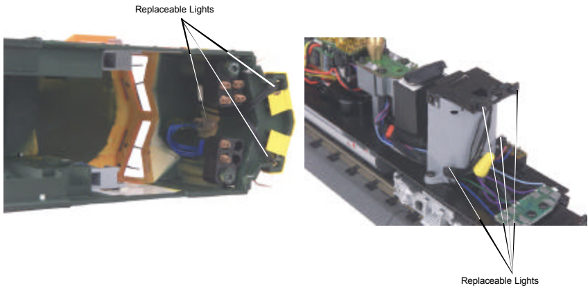
Figure 7: Removing The Replaceable Lights
