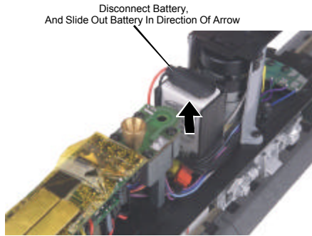
Figure 9: Removing The Battery
