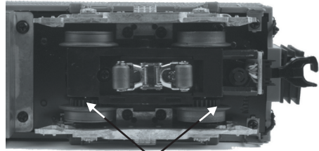
Grease Idler Gears
