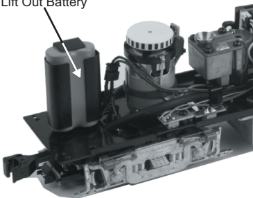
Battery Location
