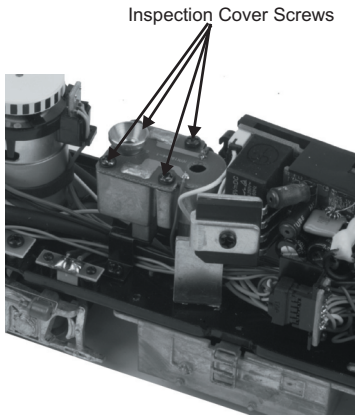
Inspecting the Smoke Unit Wick
