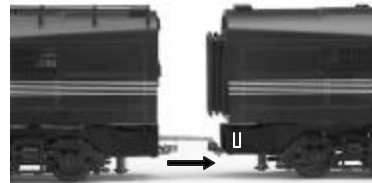
Figure 2: Connecting the two A Units together by aligning the draw bar to the pin and also align connectors to each other. Then press the two units together.
