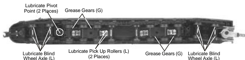
Figure 6: Lubricating The Locomotive Chassis
