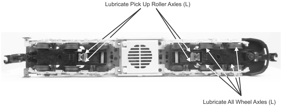
Lubrication Points on the Locomotive
