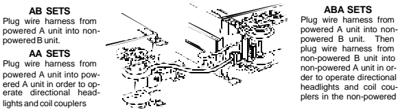
Figure 1: Plugging In the ProtoSound® Cable Harness
