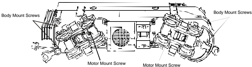
Fig. 9 Location of Body Mount Screws
