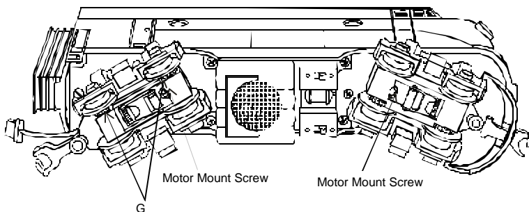
Figure 8: Greasing The Power Trucks
