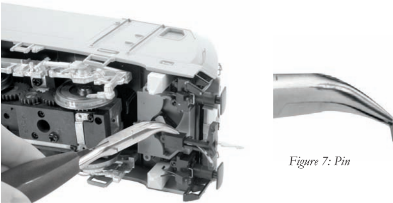
Figure 6: Removing Pin
