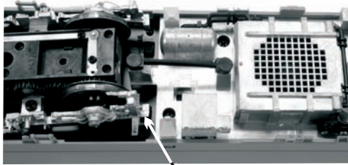
Figure 4: Pantograph/Track Position Switch
