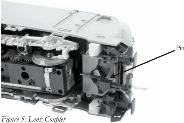
Figure 5: Lenz Coupler
