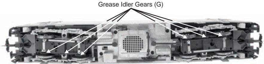
Figure 10: Greasing The Idler Gears
