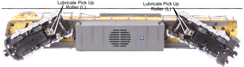
Figure 5. Lubrication Points on the Locomotive
