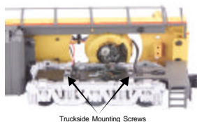
Figure 8. Truckside Mounting Screws to Access the Traction Tires
