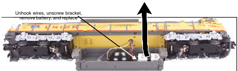
Figure 11. Replacing the Battery (Remove all four screws on the fuel tank to access the battery).
