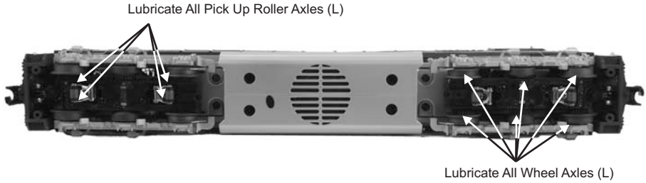
Figure 9: Lubrication Points on the Locomotive
