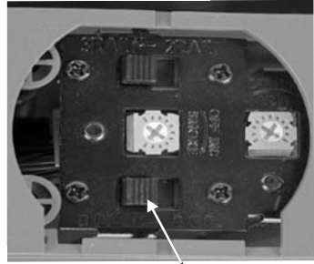
DCS/DCC Switch
