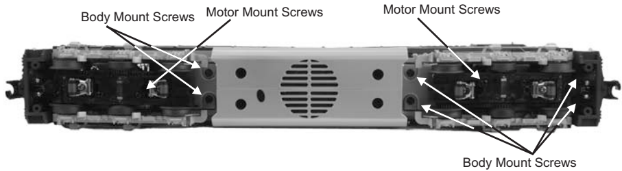
Figure 10: Body Mount Screws
