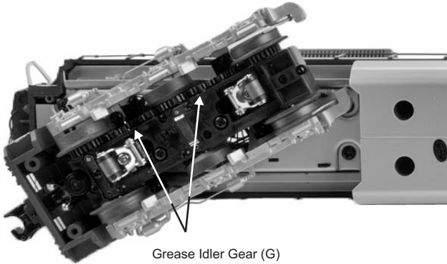
Figure 11: Greasing the Idler Gears
