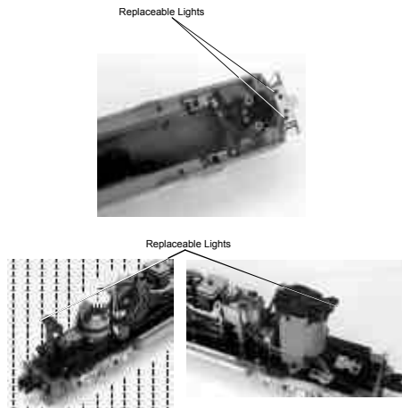
Figure 7: Removing The Replaceable Lights
