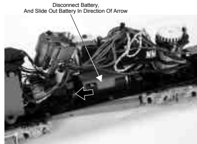
Figure 9: Removing The Battery
