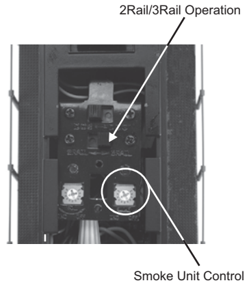
Figure: Smoke Unit Control + 2Rail/3Rail Switch
