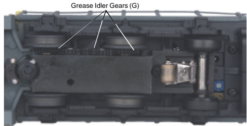
Figure 6: Greasing The Idler Gears
