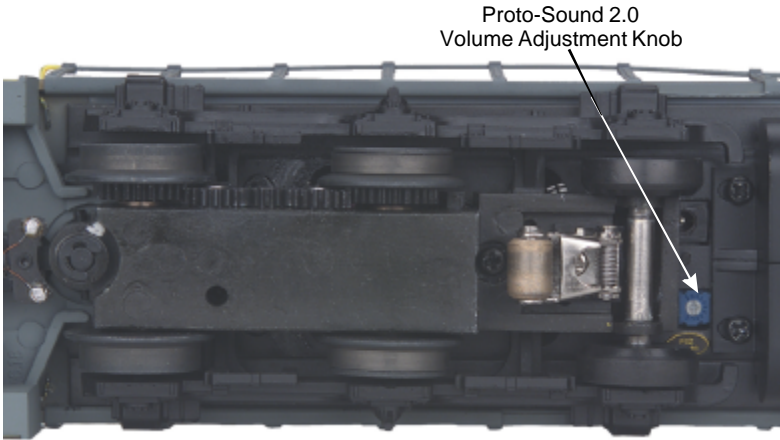
Figure 4: Manual Volume Adjustment Knob
