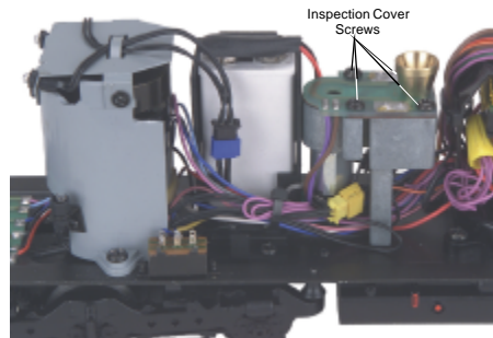
Figure 11 : Smoke Unit Inspection
