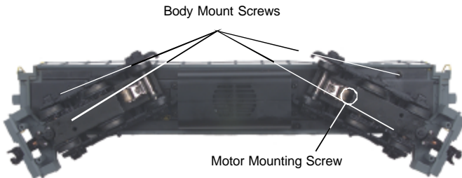
Figure 5: Body Removal Screw Locations
