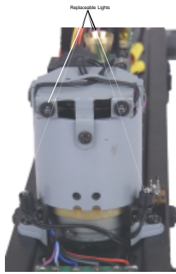
Figure 7: Removing The Replaceable Lights
