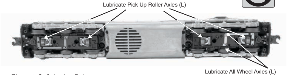
Figure 8: Lubrication Points
