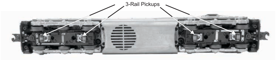
Figure 4: 3-Rail Pickups
