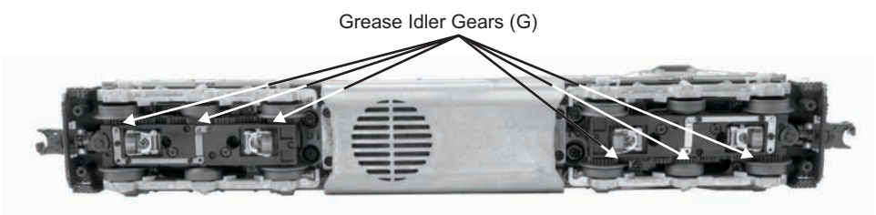
Figure 10: Greasing The Idler Gears
