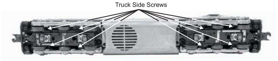
Figure 11: Truck Side Screws
