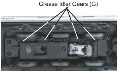
Figure 7. Greasing The Idler Gears
