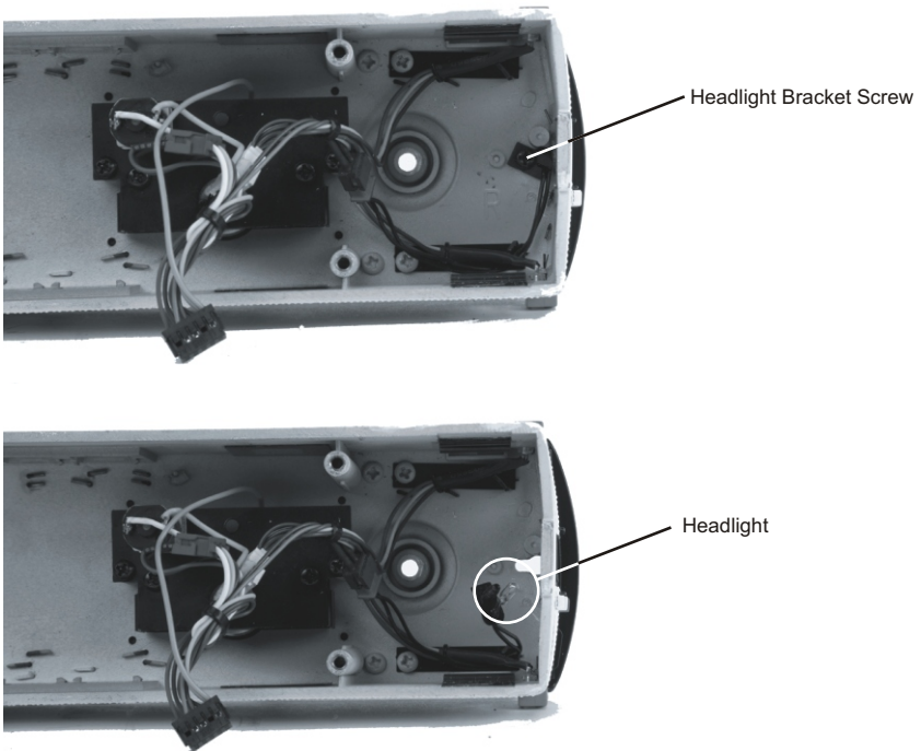
Figure 8. Removing the Headlight
