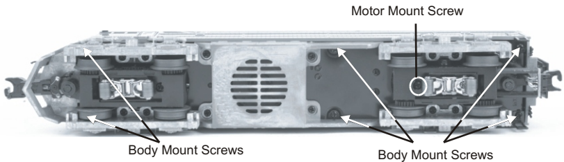
Body Removal Screw Locations
