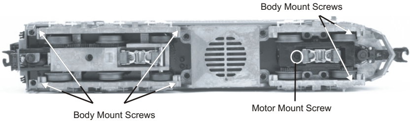
Body Removal Screw Locations
