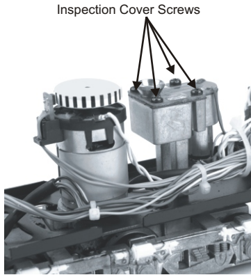
Inspecting the Smoke Unit Wick
