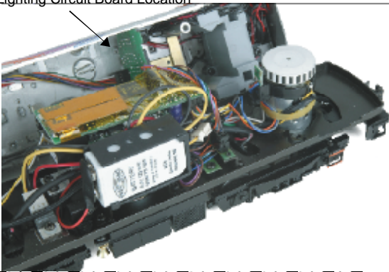
Access Lights By Removing Cab Interior Screws
