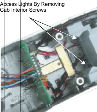
Remove Burned Out Lights By Unplugging From Circuit Board
