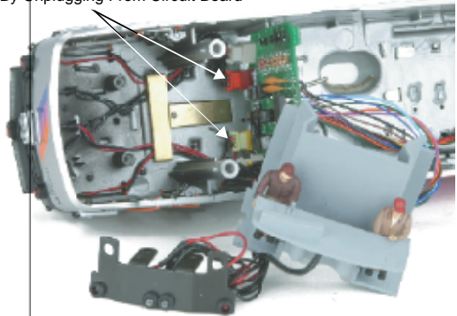
Remove Burned Out Lights By Unplugging From Circuit Board
