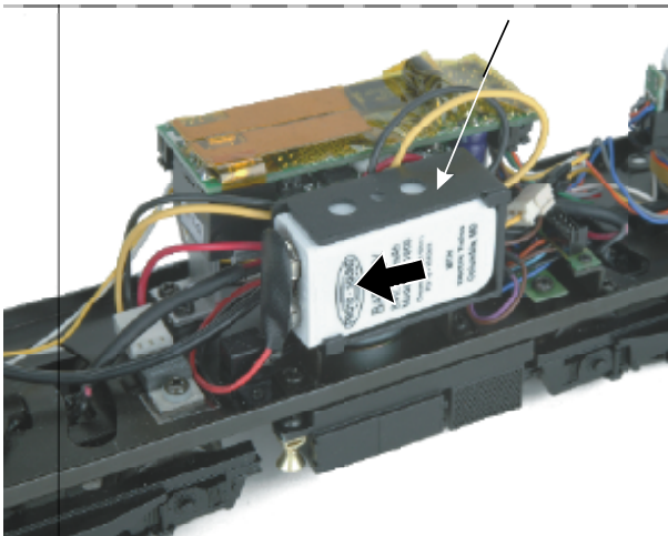
Figure 8: Removing The Battery
