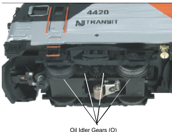
Figure 4: Oiling Idler Gears
