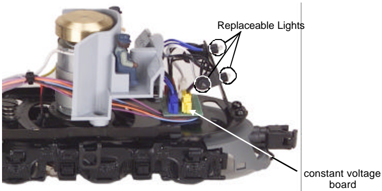
Figure 12. Locations of Replacable Lights
