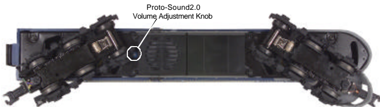
Figure 2. Proto-Sound 2.0 Volume Adjustment Knob
