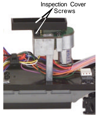
Figure 6. Inspecting the Smoke Unit
