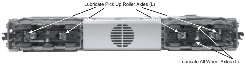
Figure 1. Lubrication Points on the Locomotive
