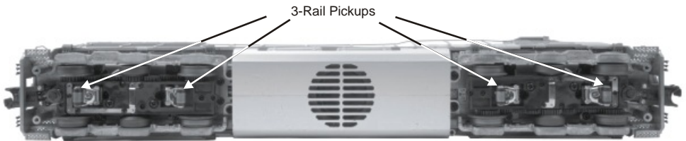
Figure 4: 3-Rail Pickups
