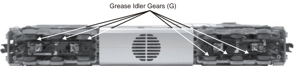
Figure 10: Greasing The Idler Gears
