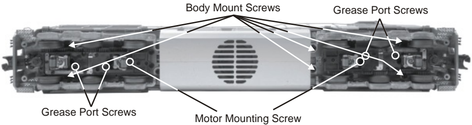
Figure 8: Lubrication Points
