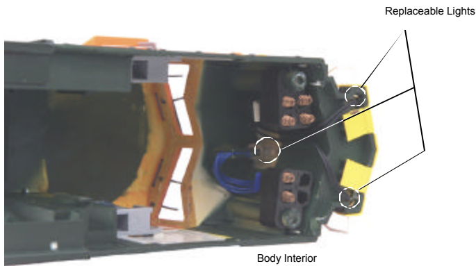
Figure 5: Removing The Replaceable Lights
