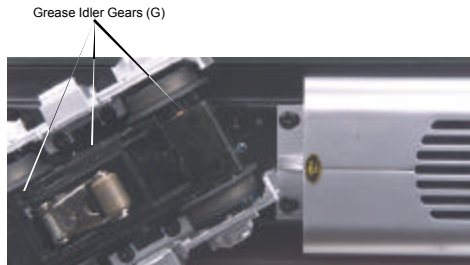
Figure 4: Greasing The Idler Gears
