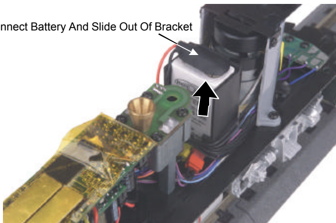
Figure 7: Removing The Battery
