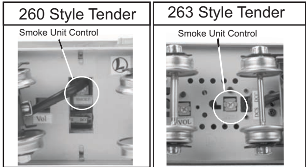
Figure 3: Smoke Unit Control
