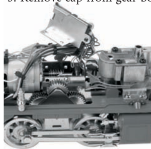
Fig. 13: Removing Cap
