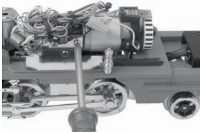
Fig. 12: Unscrewing Gearbox screws
