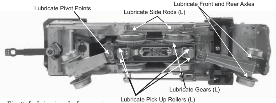
Fig. 8: Lubricating the Locomotive
