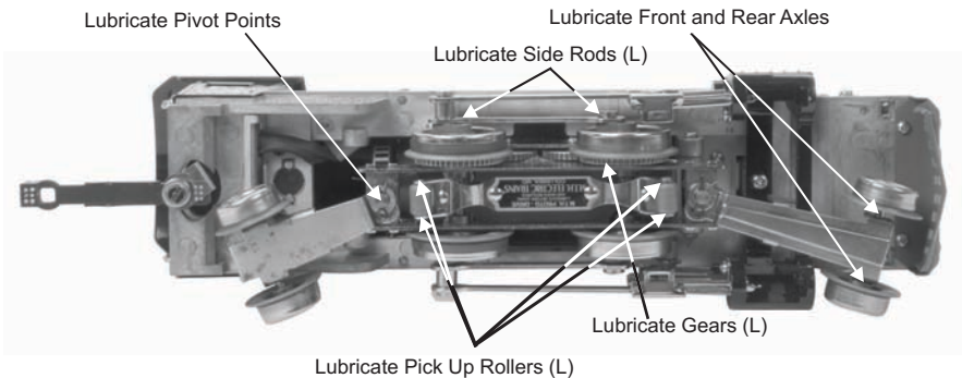
Fig. 1: Lubricating the Locomotive
