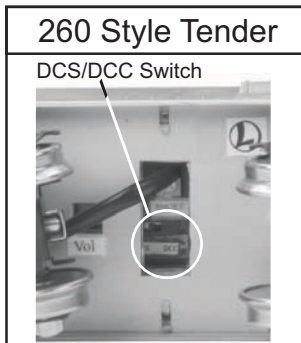
Figure 6: DCS/DCC Switch
