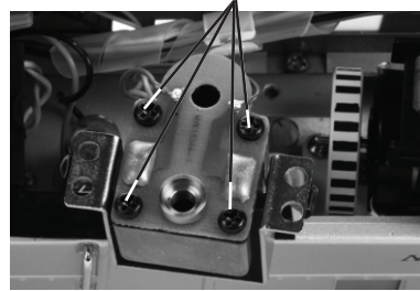
Inspection Cover Screws
