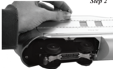
Remove Truck Block Mounting Screw
