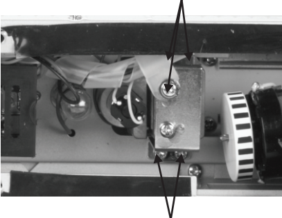
Remove Screws to Access Smoke Unit
