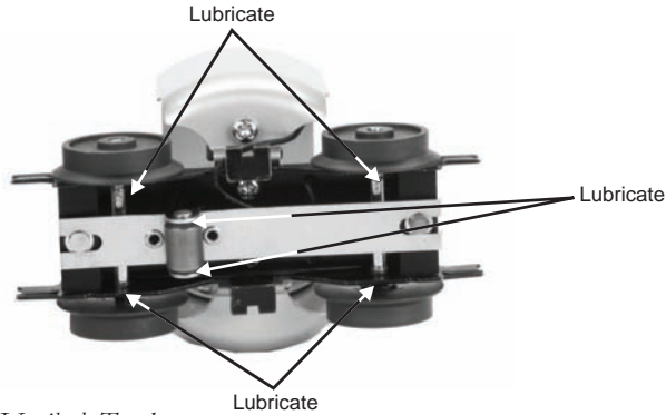
Figure 11: Lubricating Vestibule Truck
