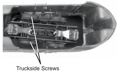
Figure 12: Traction Tires
