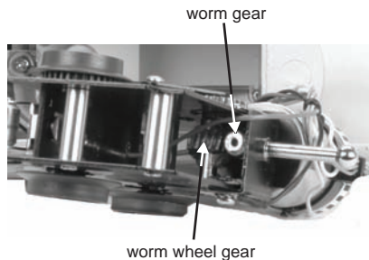
Figure 10: Grease Worm Gear
