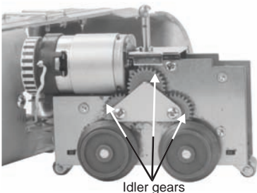
Figure 9: Grease Idler Gears
