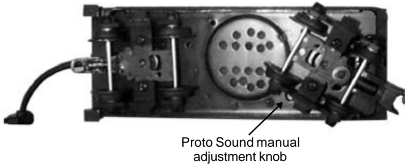
Figure 6: Adjusting The ProtoSound® Volume
