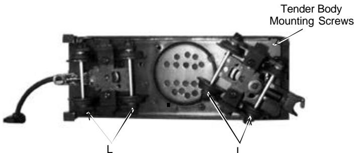
Figure 9: Lubricate The Tender Chassis Trucks
