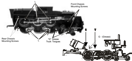
Figure 8: Lubricating The Locomotive Chassis
