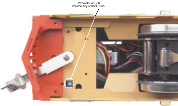
Figure 2: Manual Volume Adjustment Knob
