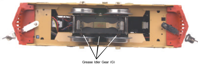
Figure 4: Greasing The Idler Gears
