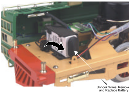
Figure 7: Removing The Battery
